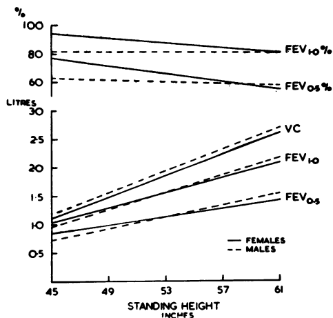
FIG. 1(a)—(lower graph)—Regression lines for absolute values of F.E.V. 0.5 , F.E.V. 1.0 and V.C. on standing height for both sexes. FIG. 1 (b).—(upper graph)—Relates values for F.E.V. 0.5 % and F.E.V. 1.0 % (calculated from regression lines in Fig. 1(a)) to standing height for both sexes.
