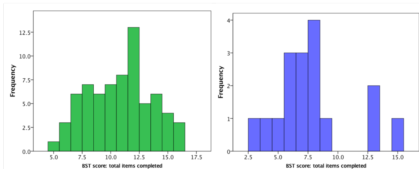
Figure 1 Histograms of Babyscreen scores (total number of items completed without visual demonstration) in those children with normal BSID-III cognitive composite scores ( >90 , n=71) in light green and in those children (n=17) with a BSID-III cognitive score \leq 90 at 18–24 months (teal blue).
